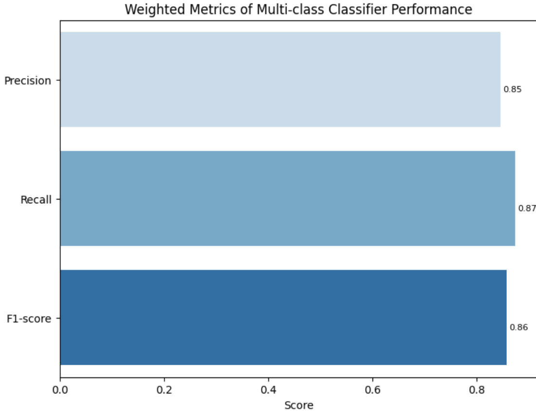
Figure 16: Model Performance Metrics
