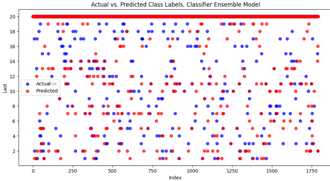
Figure 10: Ensemble Model Prediction on Validation Set
