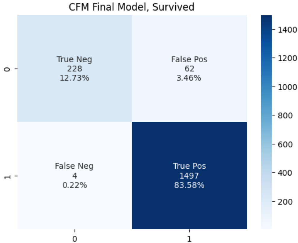
Figure 12: Ensemble Model Prediction Confusion Matrix on Validation Set
