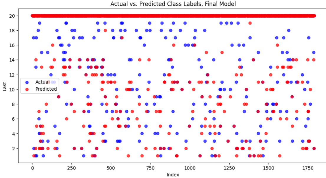
Figure 15: Final Model Survival Duration Prediction on Validation Set
