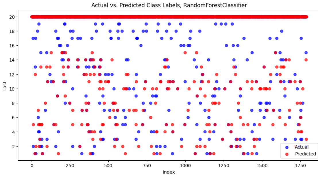
Figure 6: Random Forest Classifier Prediction on Validation Set
