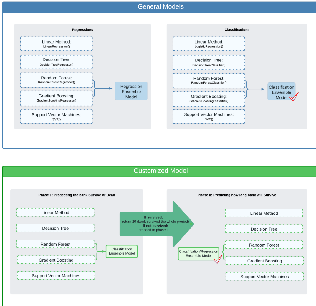
Figure 4: Modeling Workflow Diagram
