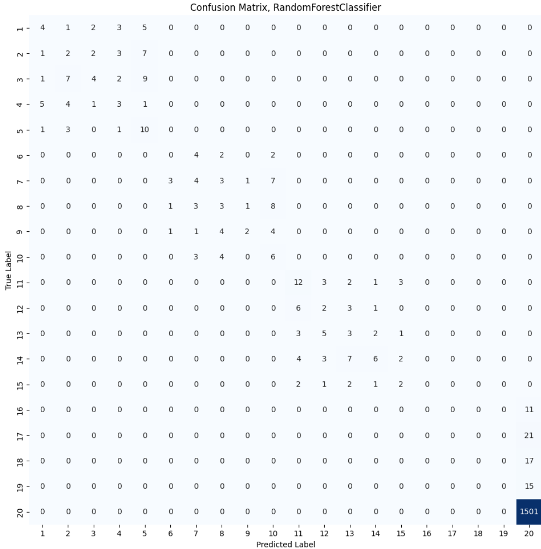
Figure 7: Random Forest Classifier Prediction Confusion Matrix on Validation Set
