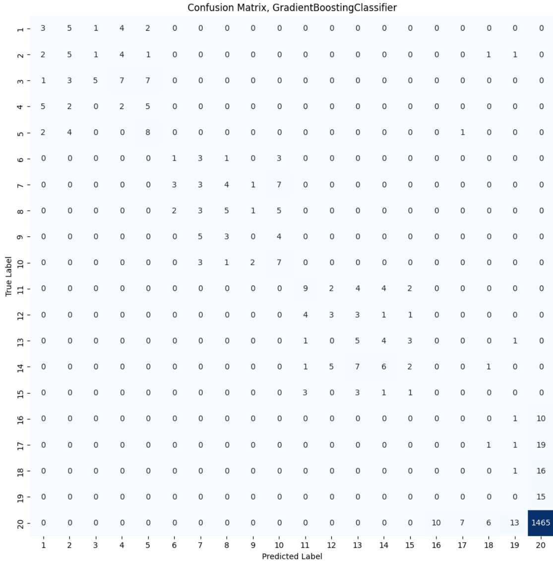
Figure 9: Gradient Boosting Prediction Confusion Matrix on Validation Set
