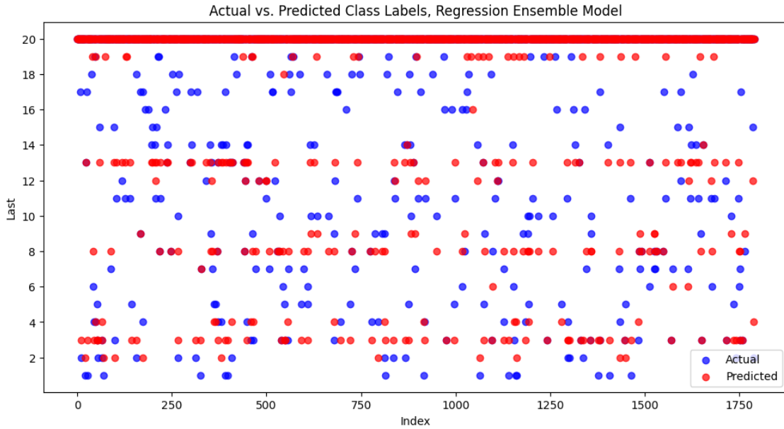
Figure 5: Ensemble Model Prediction on Validation Set
