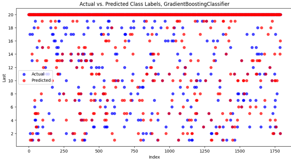
Figure 8: Gradient Boosting Prediction on Validation Set
